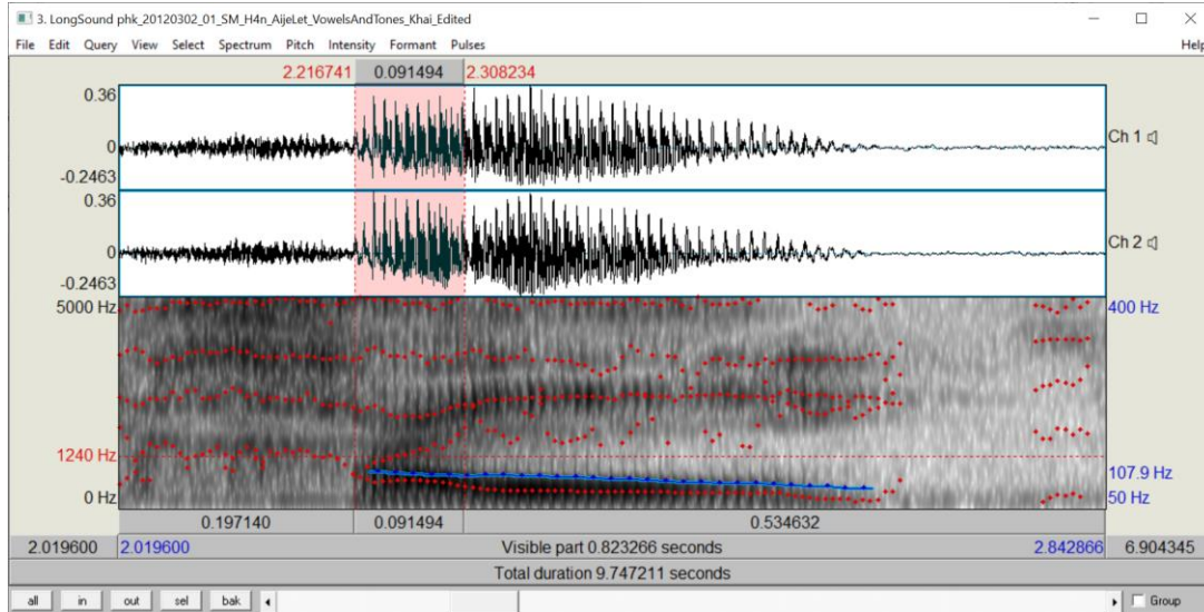
Figure 4. Wave form, pitch trace and spectrogram for the word / khai 5 / ‘tell’
